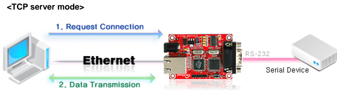
Figure 3. TCP Server mode
