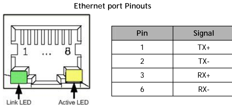
Figure 15. RJ-45 PIN Assignment
