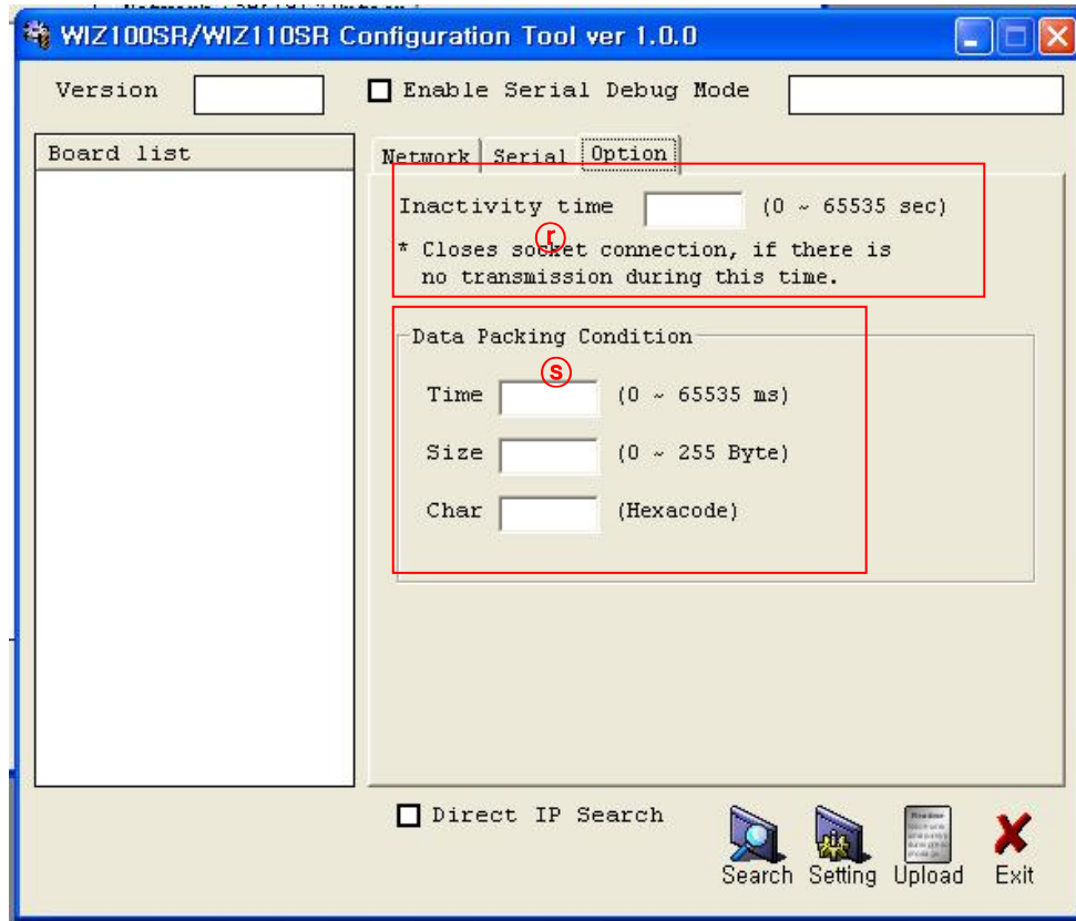
Figure 7. Configuration Tool (Option Config.)
