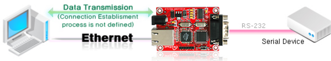
Figure 5. UDP mode
